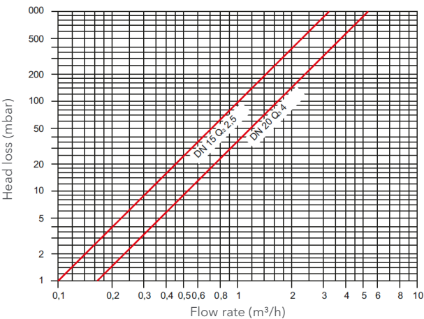
Typical Headloss Curve
